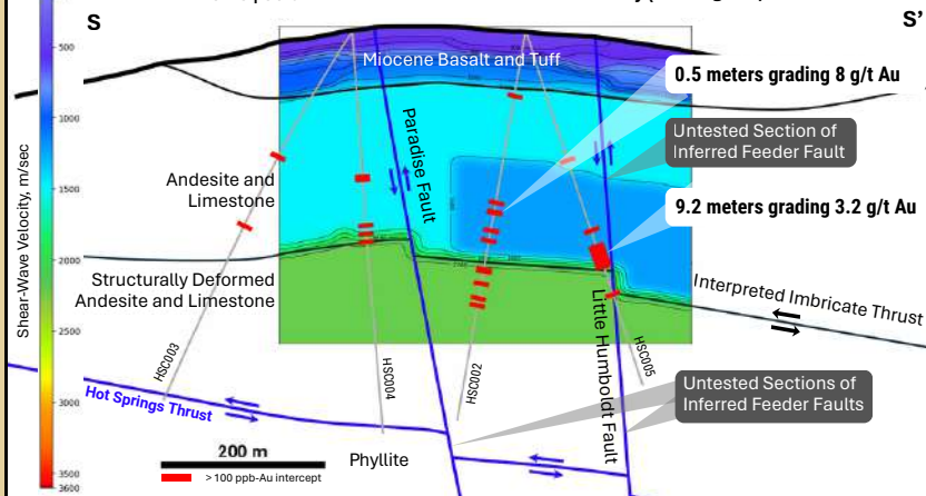
OTIS | Seismic Section S-S' with Drill Hole Overlay (Looking NW)
