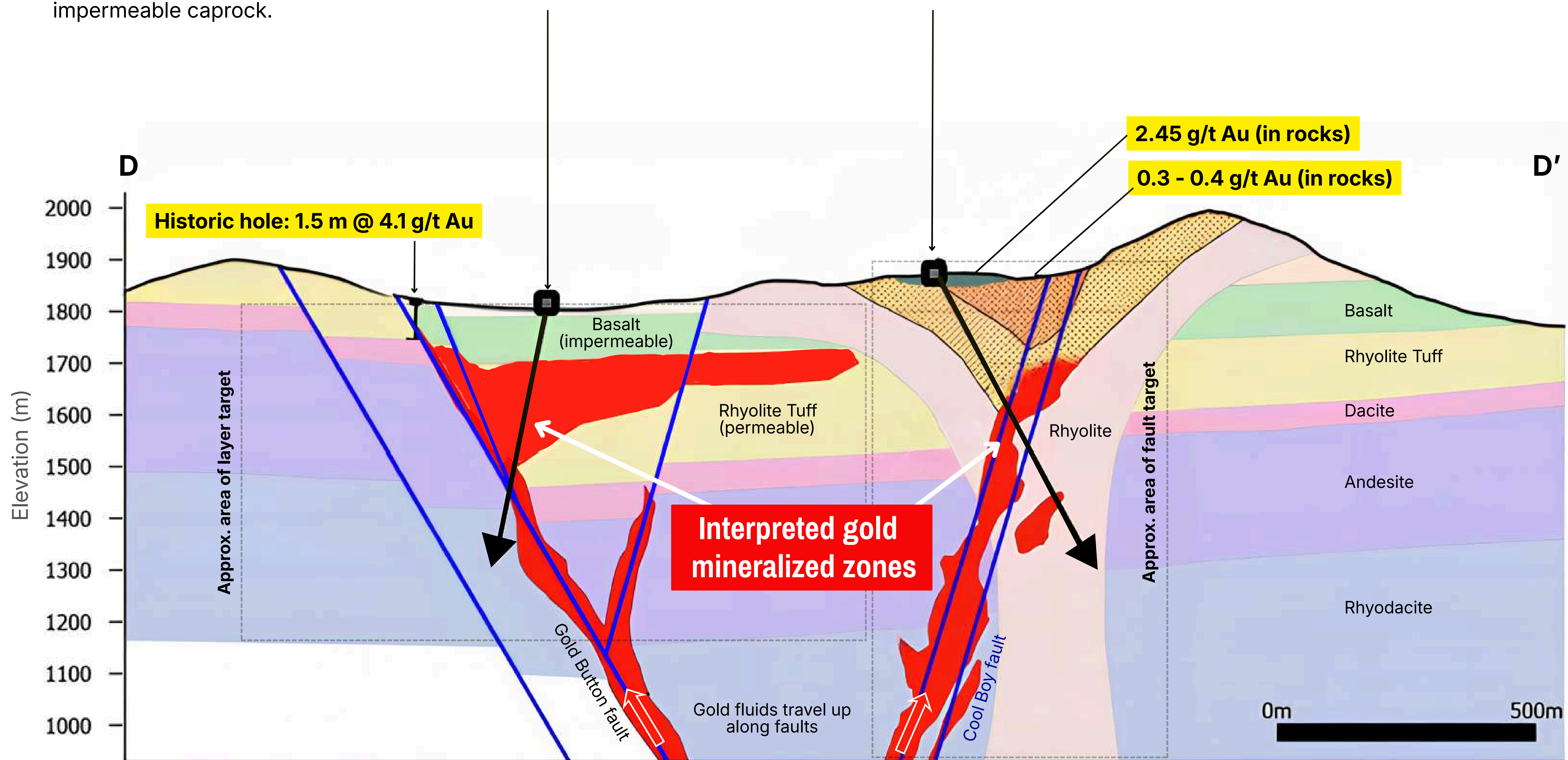
Celts: Cross Section D - D' Looking North
