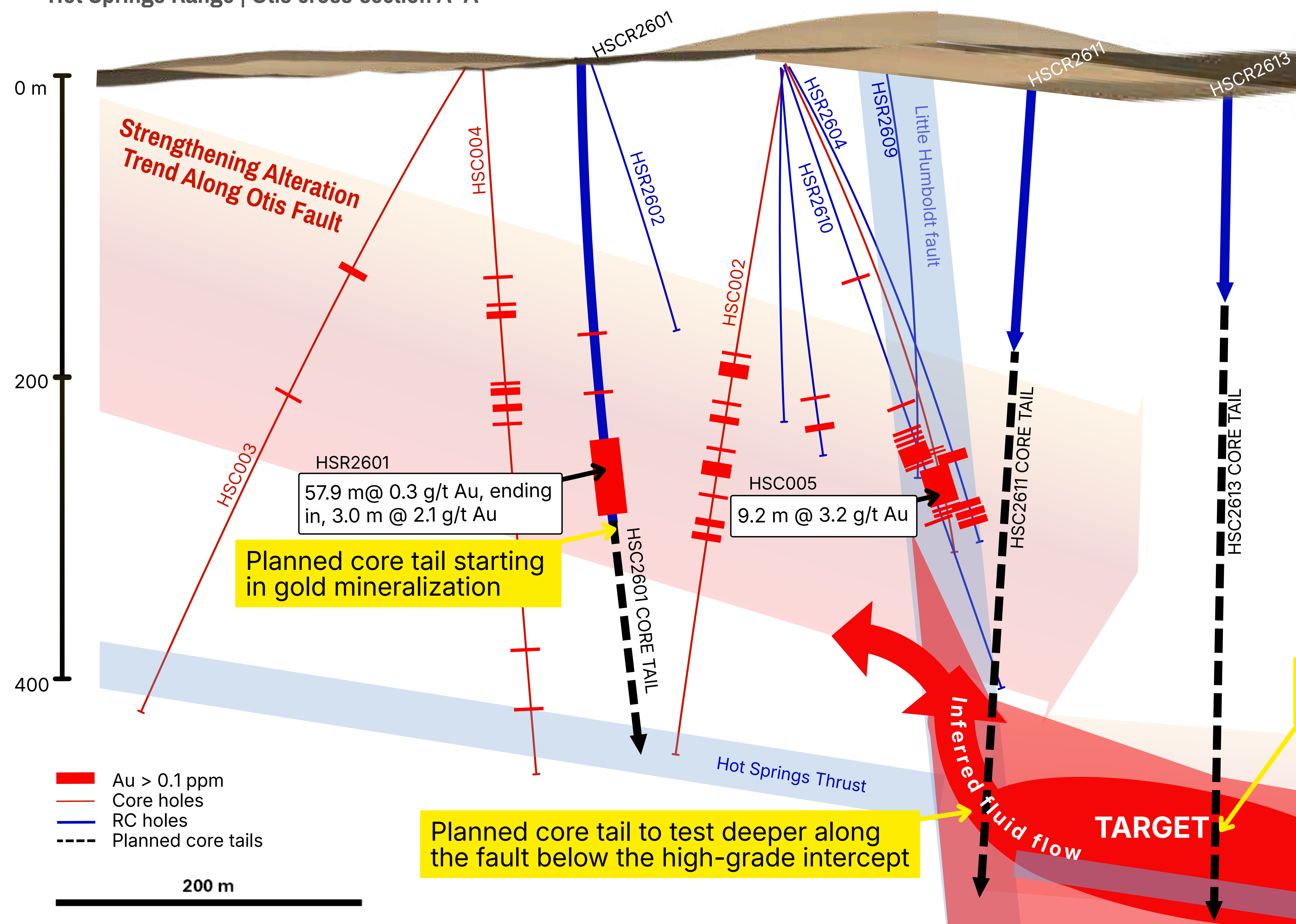
Hot Springs Range | Otis cross-section A-A'
