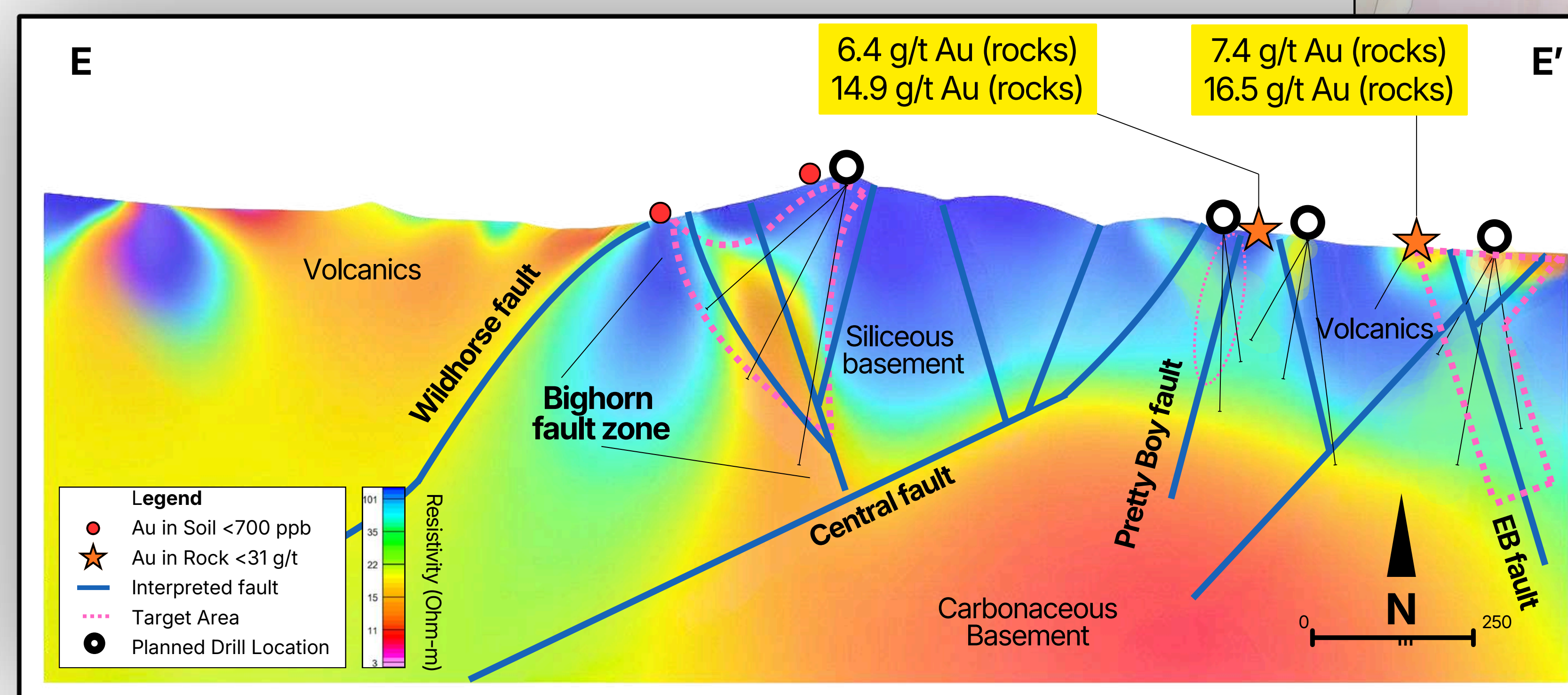
CSAMT | Gilbert South: Section D - D' Looking North
